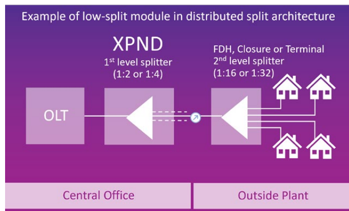
A 1:2 splitter is used in the central office with subsequent splits in the terminals/closures in the fiber infrastructure.
