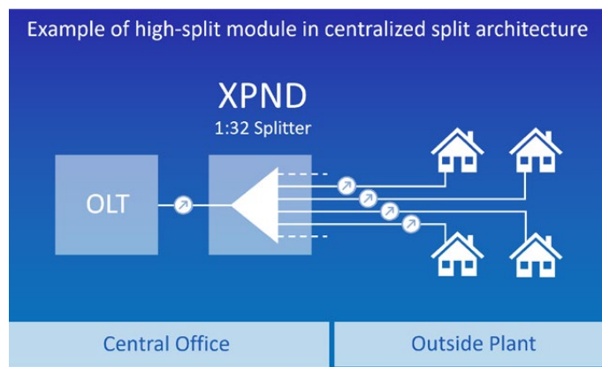
A 1:32 complete split inside and many “homerun” cables, one fiber per home, outside.
