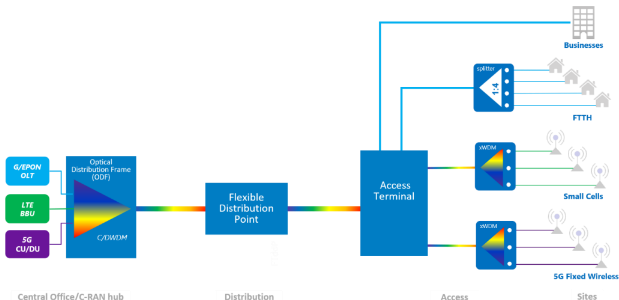
Figure 17: A WDM approach applied to the access network
