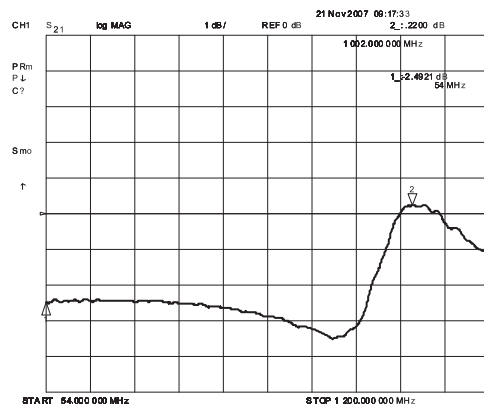
Example Peak-to-Valley Response for Peaking Circuits (727398/761843)
