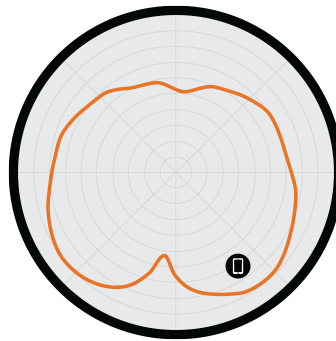
Figure 3. R350e 2.4GHz Elevation Antenna Patterns
