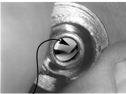
Section of ceramic sleeve broken out within the connector
